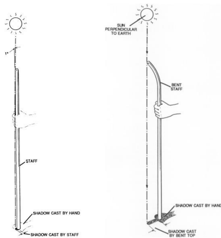
Figure 14. Use of a gnomon for the calculation of the zenith pass
